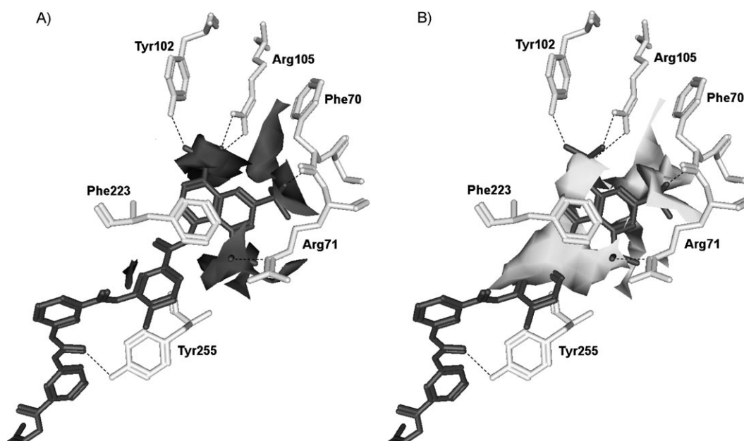
Figure 8. Favorable GRID interaction fields for the SIRT5 binding pocket (PDB code: 2NYR). Field obtained with: A) carboxyl probe (dark gray, contoured at -5.5 \text{ kcal mol}^{-1} ) and B) aromatic probe (light gray, contoured at -2.2 \text{ kcal mol}^{-1} ). Hydrogen bonds between suramin (dark gray sticks) and SIRT5 are displayed as dashed lines (black).
