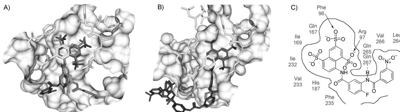
Figure 12. Docking results for suramin derivatives in the SIRT2 model. A) The two top-ranked docking solutions for compound 14a (dark and light gray atoms). B) Top-ranked docking solution for compound 5b (dark gray atoms). The additional phenyl substituent of compound 5f (light gray) as well as the other substituents of the suramin analogues 5a–5i (not shown) fit into the binding pocket. The Connolly surface (calculated with MOE) of the binding pocket is displayed. C) representation of the interaction between 14a and the SIRT2 model. Hydrogen bonds between inhibitor and enzyme are marked by arrows.
